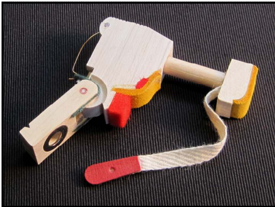
A new Asian-design hammer butt / flange assembly ready to install.
